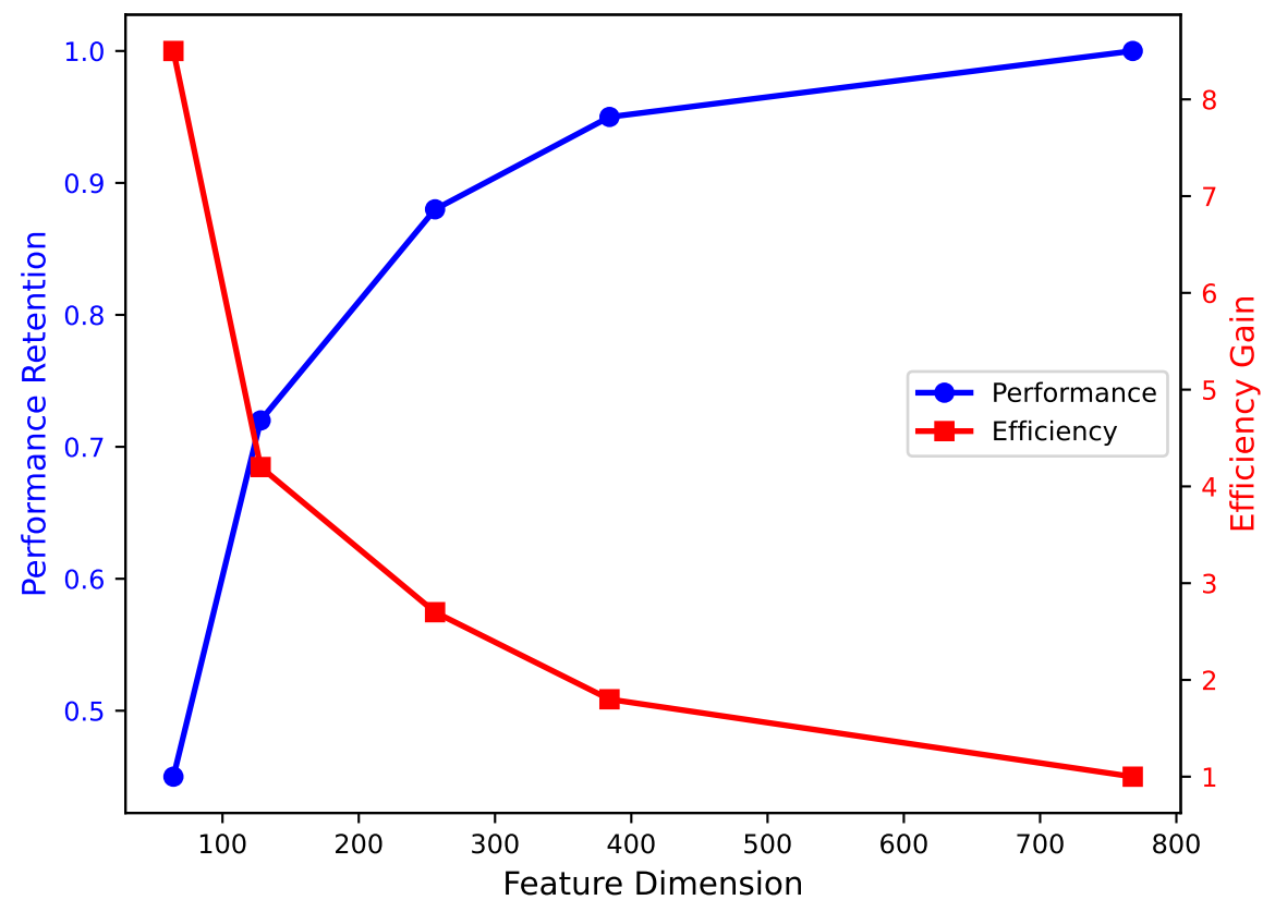
Dimension Reduction Trade-offs
